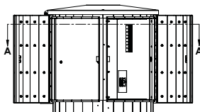
FRONT VIEW (DOORS OPEN)
