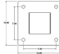
Standard Base
