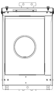
FRONT VIEW (COVER UP)
