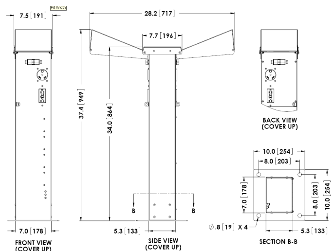
TYPICAL RVPD3 CONFIGURATION
